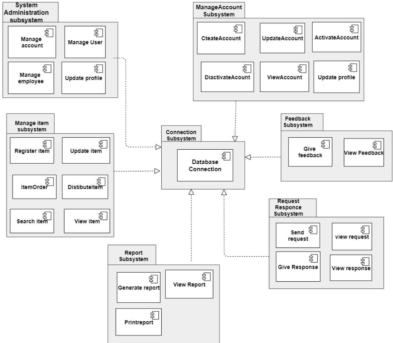
Figure 5. 2 Component diagram
