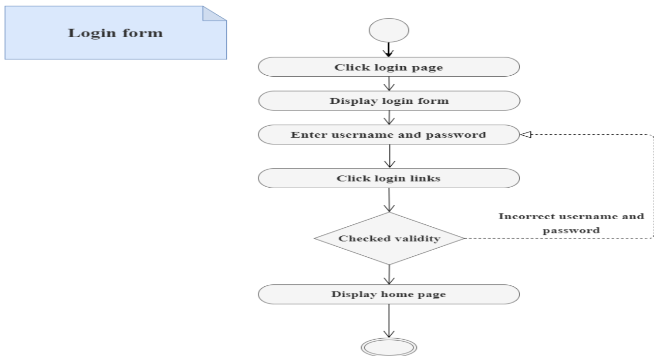
Figure 4. 6 Activity diagram for login
