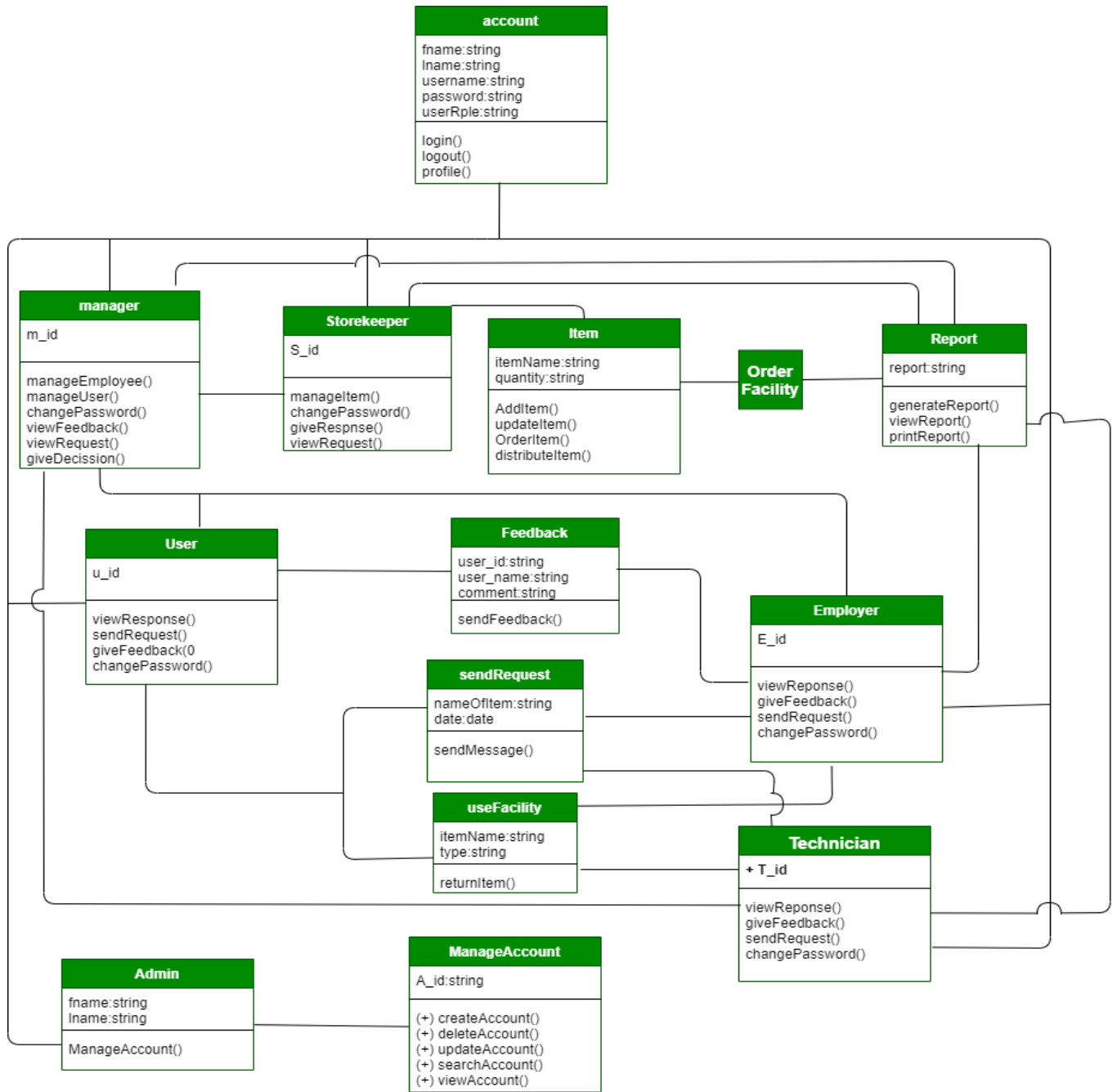
Figure 4. 2 Class diagram
