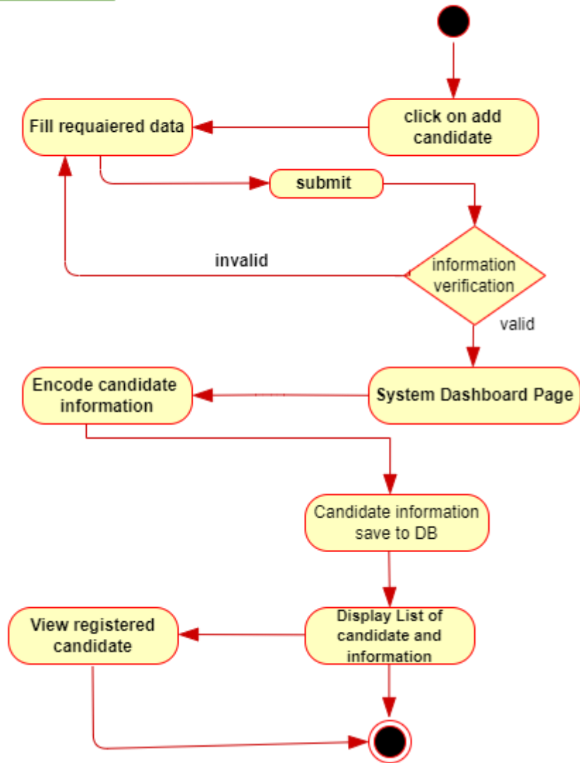
Figure 4.17 Activity Diagram for Register Candidate
