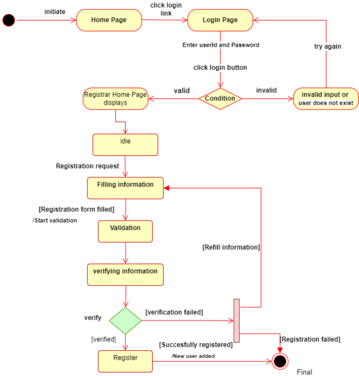
Figure 4.23 State chart Diagram for Register Candidate
