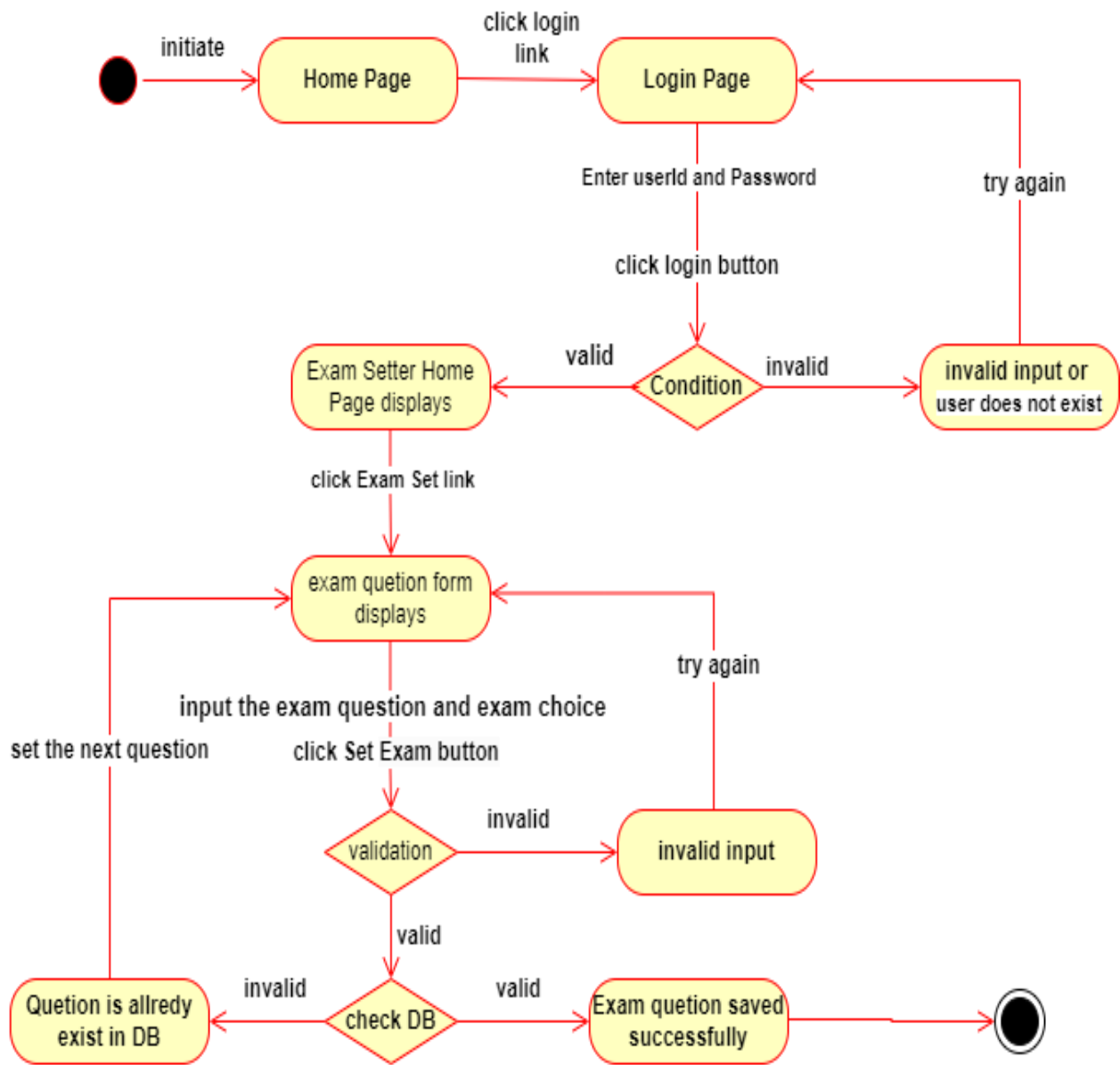
Figure 4.20 State chart Diagram for Create Set Exam
